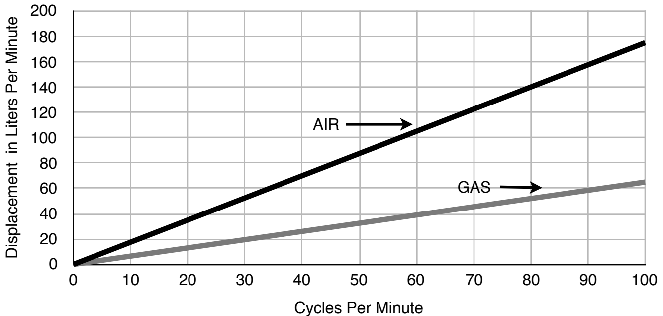
425 Models - Air and Gas Displacement vs. Cycle Rate
