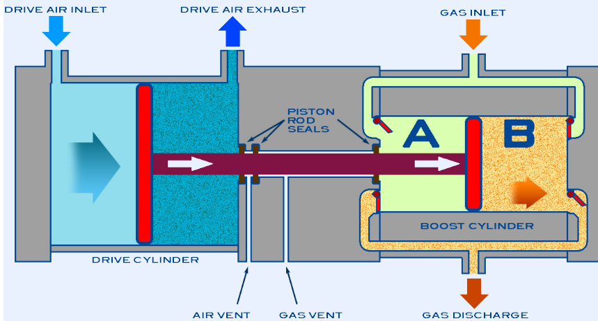
The pistons are traveling to the right and compressing the gas in chamber "B" while pulling gas into chamber "A".
