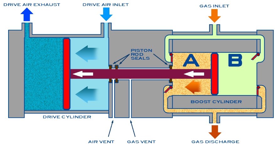
The pistons are traveling to the left and compressing the gas in chamber "A" while pulling gas into chamber "B".
